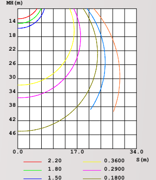
CO PLANE ISOLUX DIAGRAM (UNIT: lx)
