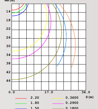
CO PLANE ISOLUX DIAGRAM (UNIT: 1x)
