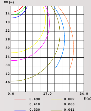
CO PLANE ISOLUX DIAGRAM (UNIT: lx)
